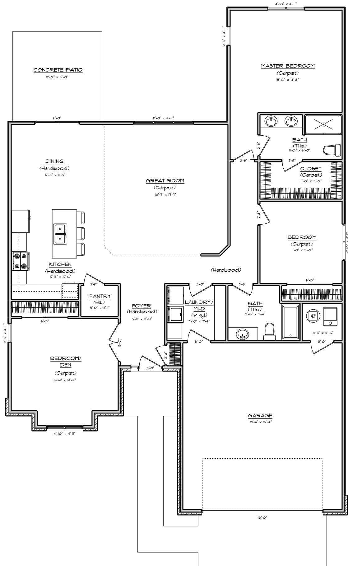
PLAN TYPE B - The Naples First Floor Plan with Crawl Space 1790 sq. ft. SCALE: \frac{1}{4}'' = 1'-0''
