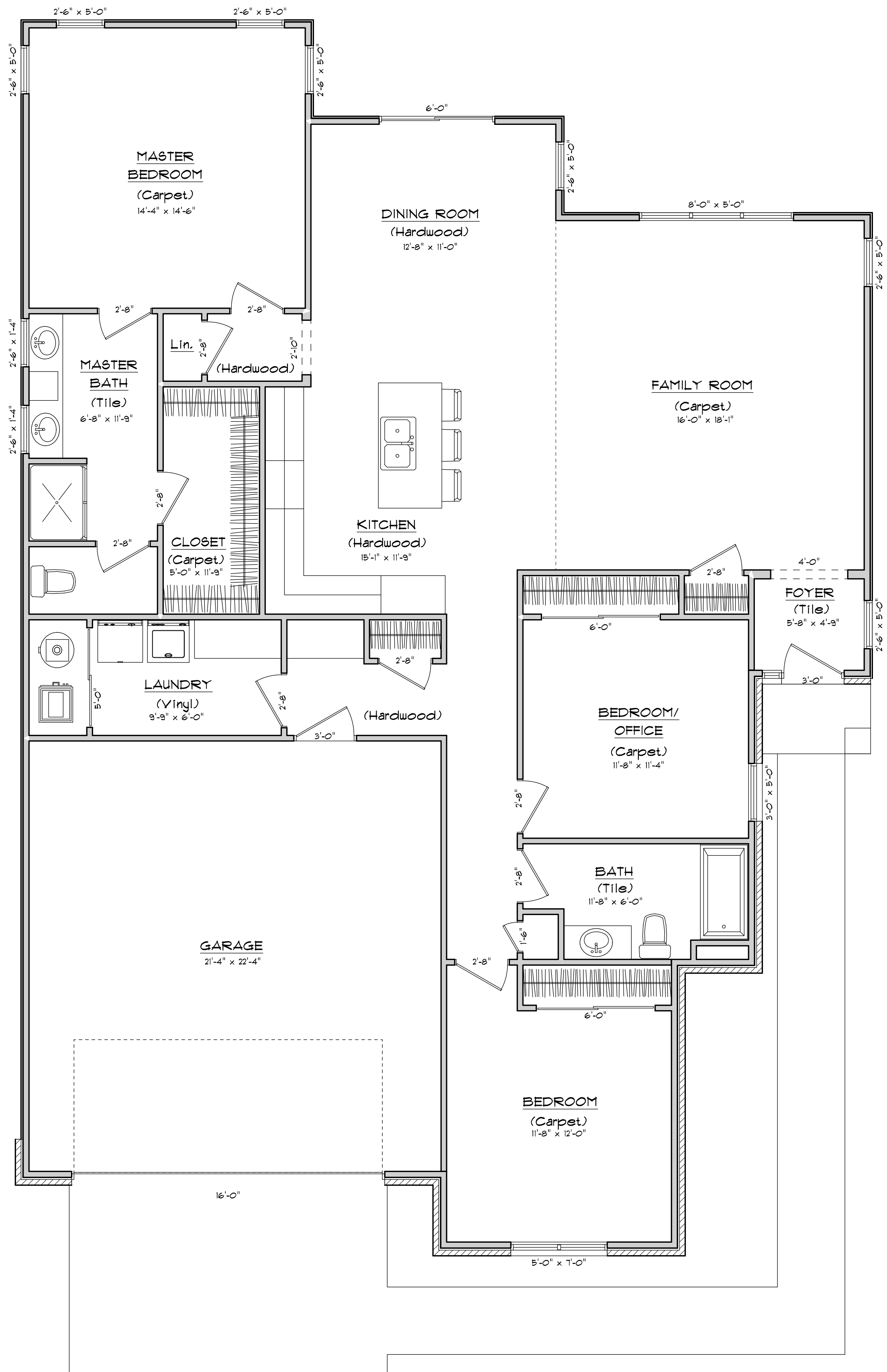
PLAN TYPE E - The Nantucket First Floor Plan with Crawl Space 1796 sq. ft.
